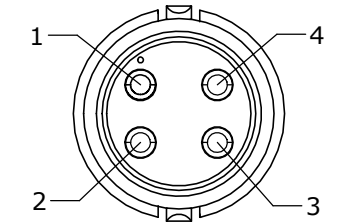
WIRE VIEW 6282-3PG-3XX SHOWN
