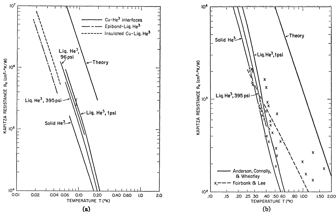
FIG. 8. (a) Experimental data on Kapitza resistance for: Cu-liquid- ^3\text{He} , Cu-solid- ^3\text{He} , Epibond 100-A-liquid- ^3\text{He} , and Formex-insulated-Cu-wire-liquid- ^3\text{He} interfaces. The data on Cu-liquid- ^3\text{He} and Cu-solid- ^3\text{He} interfaces are taken from Ref. 7, the data on the Epibond 100-A-liquid- ^3\text{He} interface are taken from Ref. 58, and the data on the Formex-insulated-Cu-wire-liquid- ^3\text{He} interface are taken from Ref. 60. The curve for theory comes from Eq. (3) applied to a Cu-liquid- ^3\text{He} interface, as calculated in Ref. 7. It is discussed in Sec. III.C. (b) Experimental data on Kapitza resistance for Cu-liquid- ^3\text{He} and Cu-solid- ^3\text{He} interfaces. The data represented by the unbroken curves are taken from Ref. 7. The points marked \times are data points of Refs. 53 and 54 on Cu-liquid- ^3\text{He} interfaces, and the broken curve is a rough fit to these data. The curve for theory comes from Eq. (2) applied to a Cu-liquid- ^3\text{He} interface, as calculated in Ref. 7. It is discussed in Sec. III.C. [Notice that (a) and (b) are drawn to different scales.]
