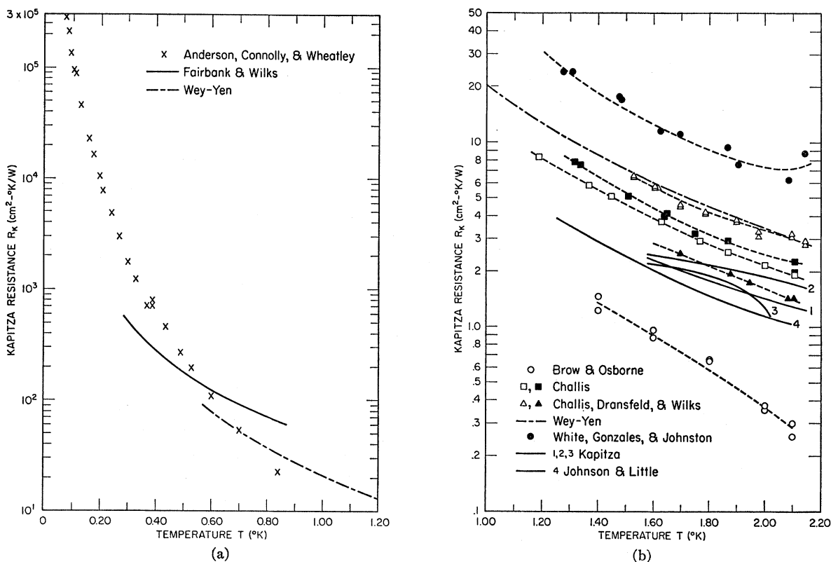
FIG. 2. (a) Experimental data on Kapitza resistance for Cu-He II interfaces from 0^\circ to 1.2^\circ\text{K} . These data are taken from Refs. 3, 4, and 7. (b) Experimental data on Kapitza resistance for Cu-He II interfaces from 1.0^\circ\text{K} to T_\lambda . These data are taken from Refs. 1, 4, 8, 9, 12, 13, and 17. The data of Challis include measurements on surfaces of work hardened Cu ( \square ), and of annealed Cu ( \blacksquare ). The data of Challis, Dransfeld, and Wilks include measurements on polished Cu ( \triangle ) and on surface-etched Cu ( \blacktriangle ). The solid curves labeled 1, 2, 3 are from Kapitza's original experiments. Curve 1 is for polished Cu, curve 2 is for Cu with a surface layer of varnish, and curve 3 is for Cu surrounded by emery powder. The solid curve labeled 4 is from measurements of Johnson and Little on an oxidized Cu surface.
