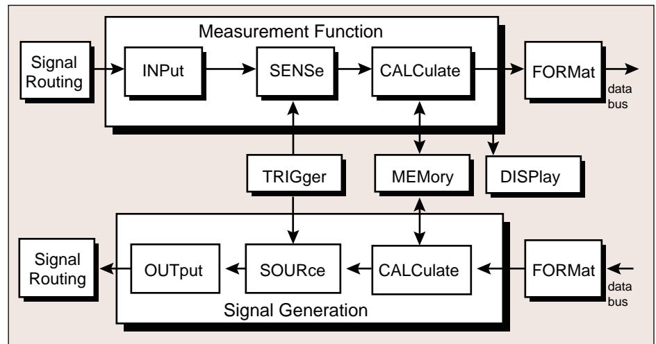
Figure 10. The SCPI Instrument Model
