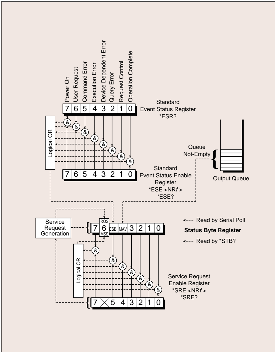
Figure 9. IEEE 488.2 Status Report Model
