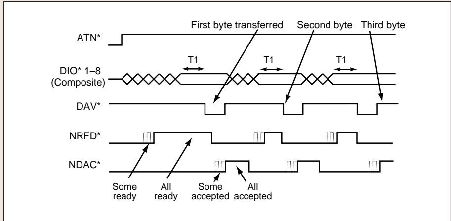
Figure 7. Normal IEEE 488.1 Handshake
