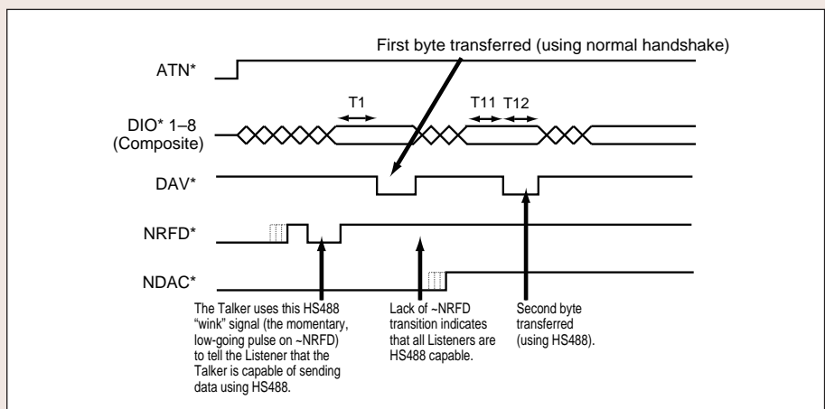
Figure 8. HS488 Handshake
